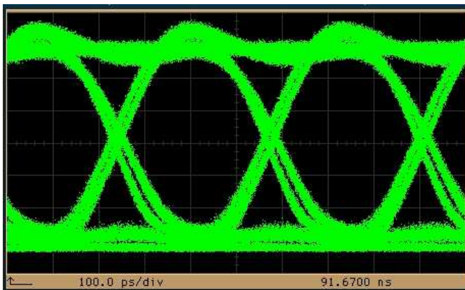
3.0Gbps PN31 2V/div
